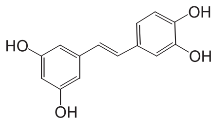
Fig. 1. Structure of Piceatannol
